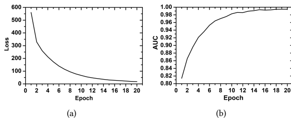
Figure 5: Training loss and the AUC curves.
